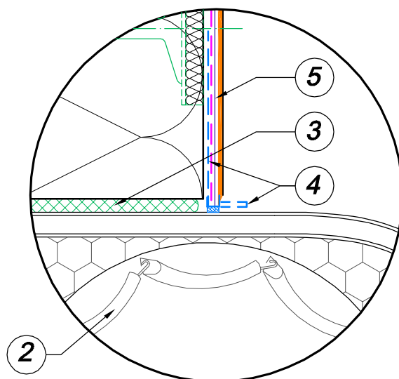
No. 1.3.9 Lintel insulation with external window blind
