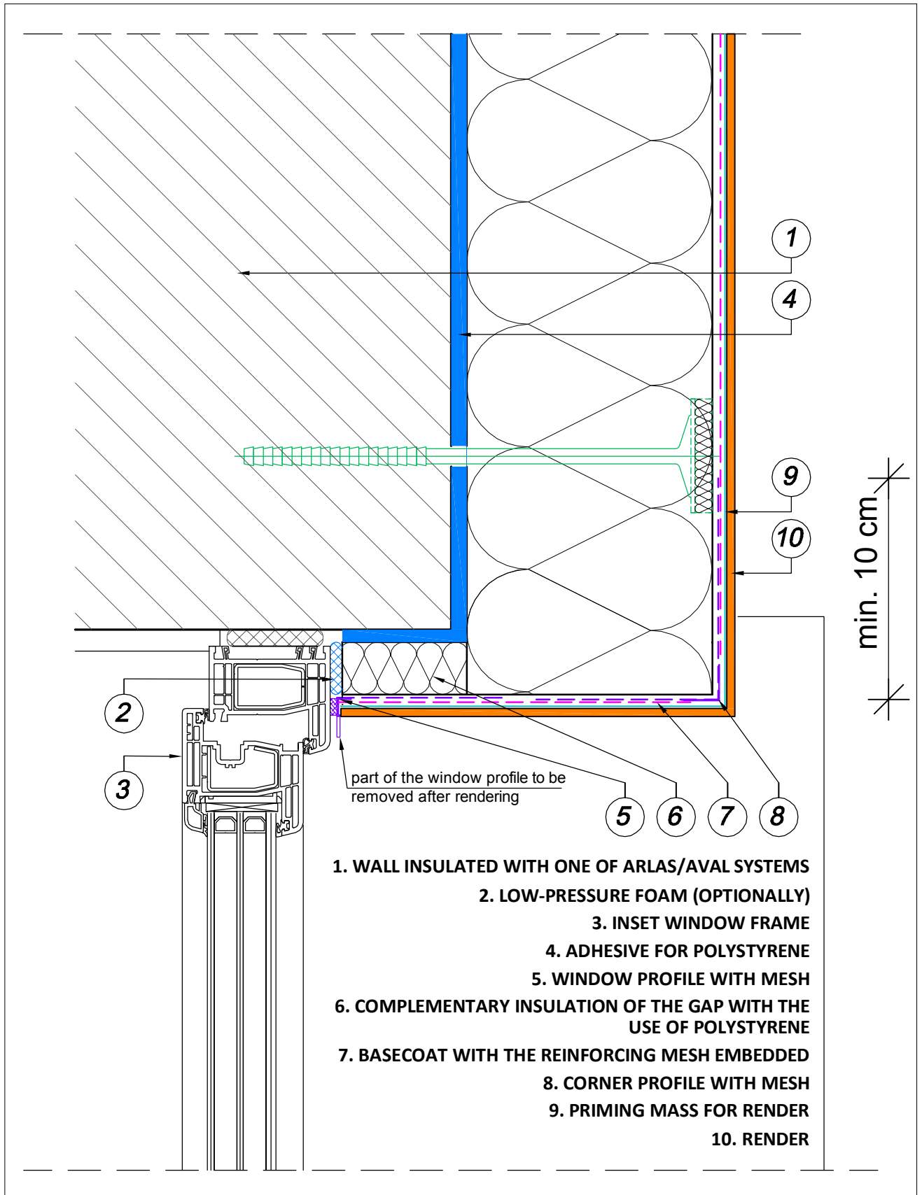
No. 1.3.7 Inset reveal insulated with the use of window profile - detail
