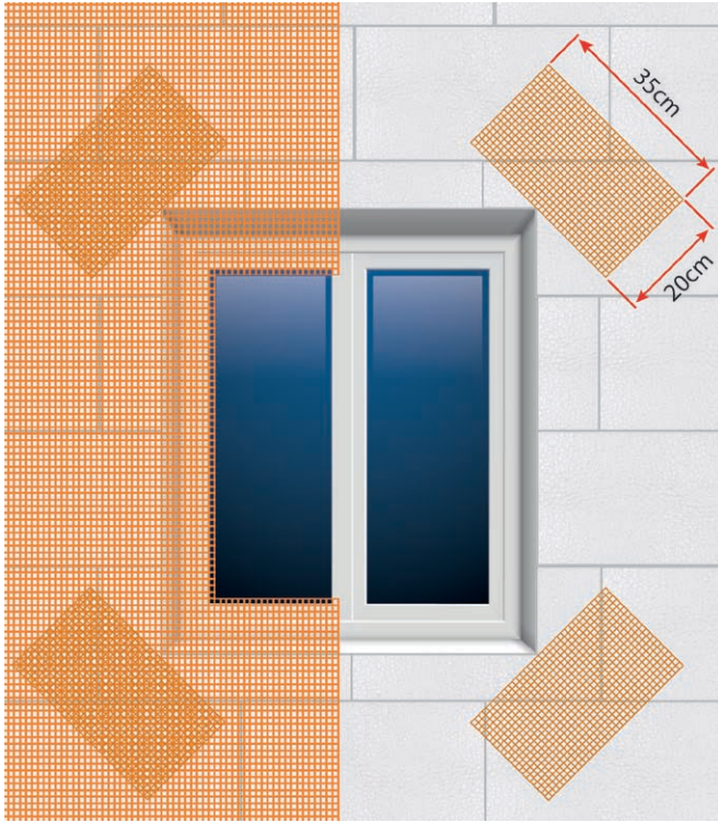
PREPARATION OF THE WINDOW REVEAL WITH THE USE OF CORNERS AND DIAGONALLY APPLIED MESH STRIPS
