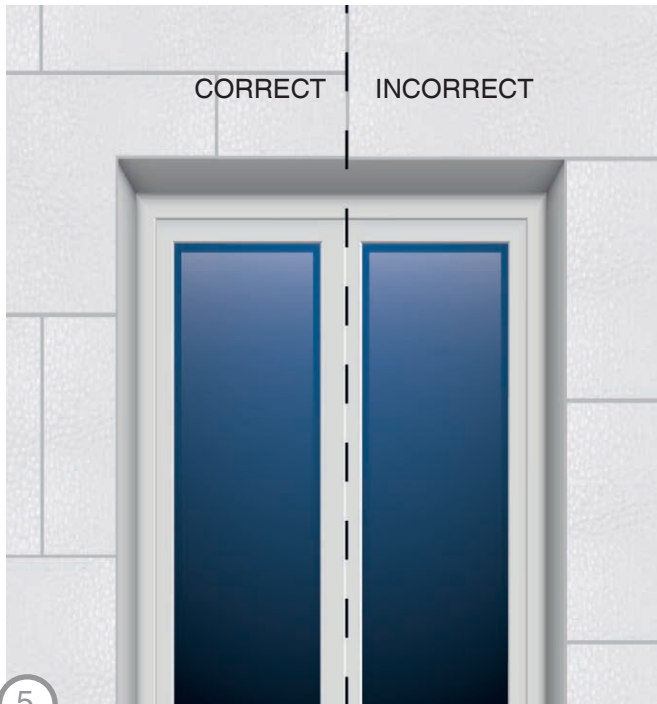
5 CORRECT AND INCORRECT ARRANGEMENT OF POLYSTYRENE BOARDS IN WINDOW REVEALS
