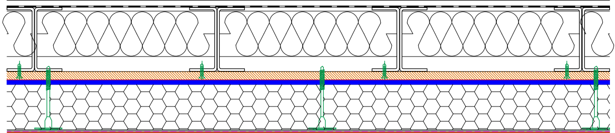
EXTERNAL WALL INSULATION SYSTEM WITH EXPANDED POLYSTYRENE (EPS) ON A SUBSTRATE MADE OF ORIENTED STRAND BOARD (OSB) BASED ON A STEEL FRAME STRUCTURE
