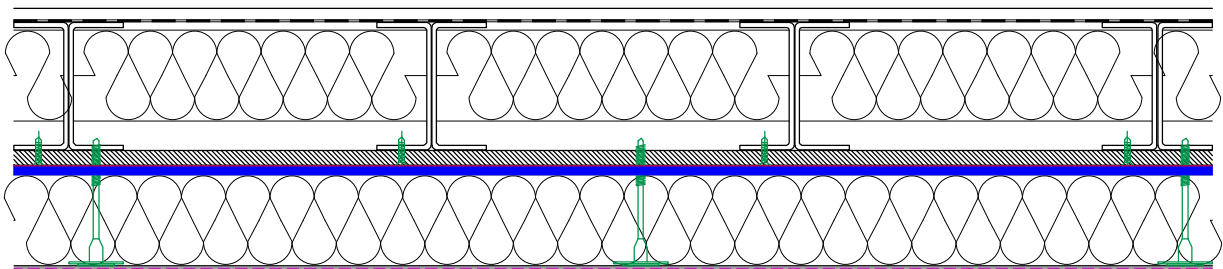
EXTERNAL WALL INSULATION SYSTEM WITH MINERAL WOOL (MW) ON A SUBSTRATE MADE OF FIBRE CEMENT BOARD (FCB) BASED ON A STEEL FRAME STRUCTURE
