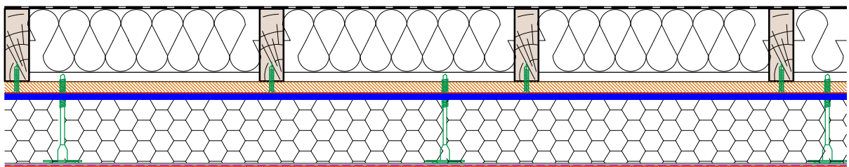
EXTERNAL WALL INSULATION SYSTEM WITH EXPANDED POLYSTYRENE (EPS) ON A SUBSTRATE MADE OF ORIENTED STRAND BOARD (OSB) BASED ON A TIMBER FRAME STRUCTURE
