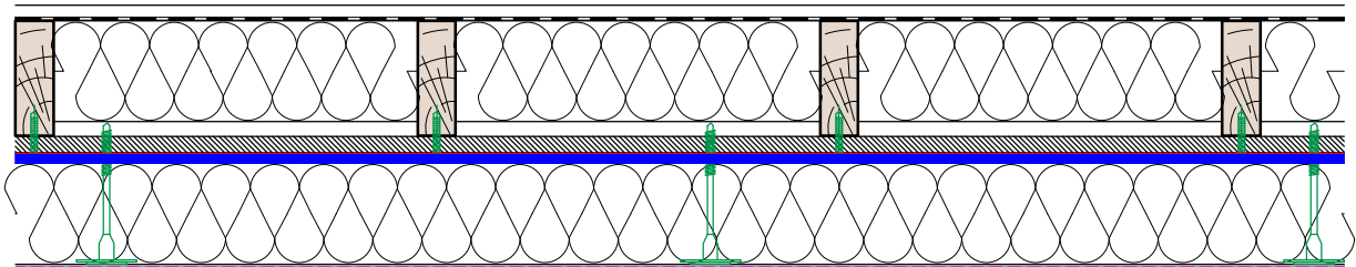
EXTERNAL WALL INSULATION SYSTEM WITH MINERAL WOOL (MW) ON A SUBSTRATE MADE OF FIBRE CEMENT BOARD (FCB) BASED ON A TIMBER FRAME STRUCTURE
