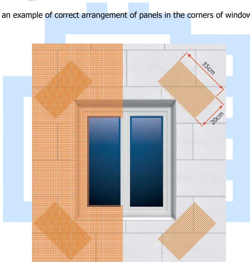
places for installing additional diagonal reinforcements
